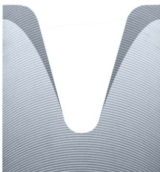
Bottom tool with WILA's proprietary CNC-Deephardening® process applied.
